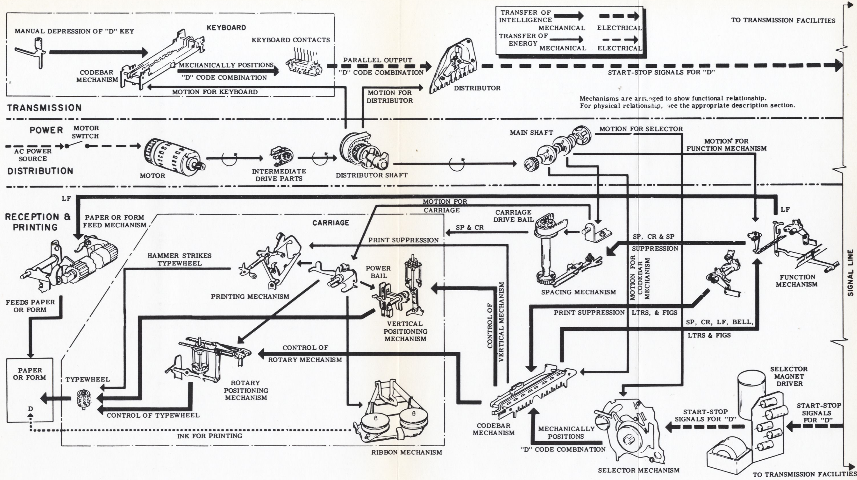
Figure 3 - Schematic Diagram - Typing Unit Operation
