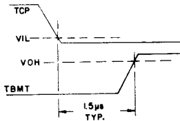
Fig.42 TBMT TURN-ON
