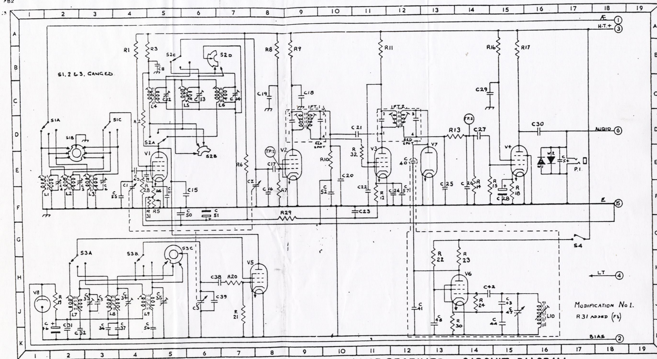
MK.123.RECEIVER - CIRCUIT DIAGRAM
