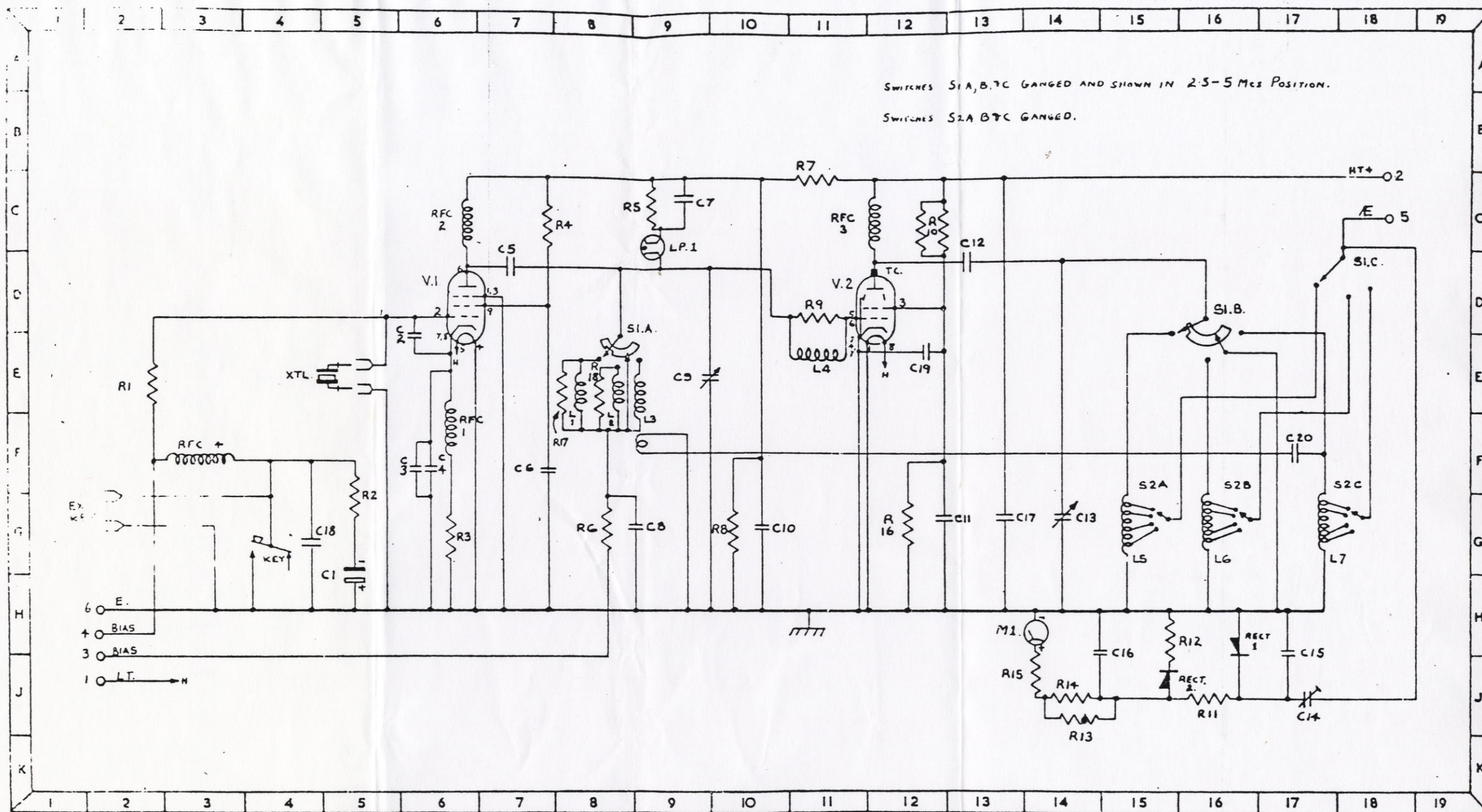
MK.123. TRANSMITTER - CIRCUIT DIAGRAM
