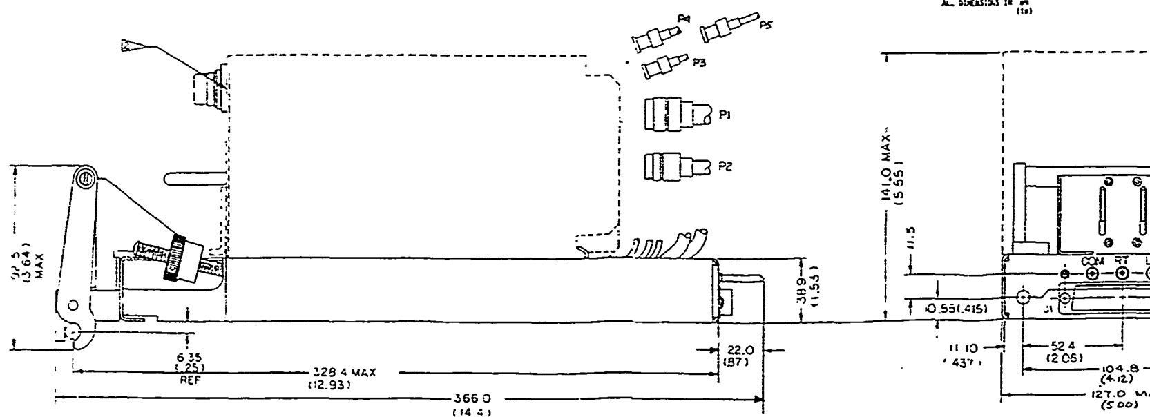
FIGURE 4-3 1-8 Installation Control Drawing, Adapter Tray MT-6373 with RT-1477A
