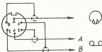
Plug 11-1-0-0 per TGL 24685 (soldering side)
