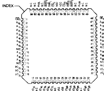
64 PIN VQFP (top view)
