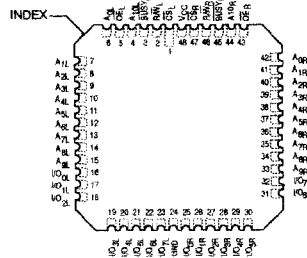
48 PIN PLCC (top view)
