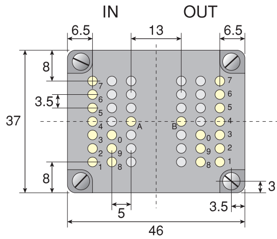
Contact block (bottom view)
