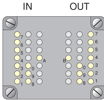
Contact block (bottom view)
