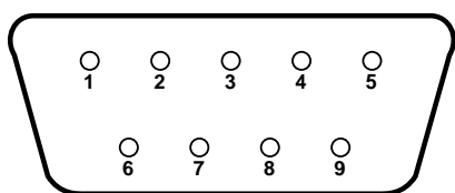
MALE 9 PIN SUBMINIATURE D CONNECTOR
