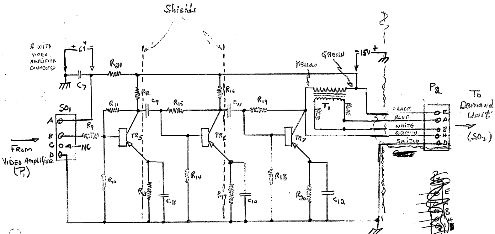
Audio Amplifier Figure #7
