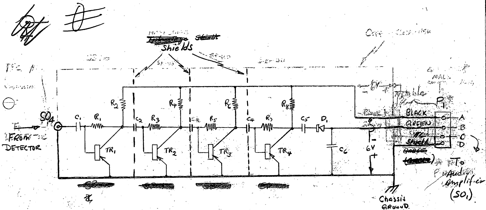
VIDEO Amplifier Figure #6
